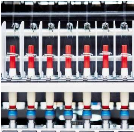
FLUTTED ROLLER
